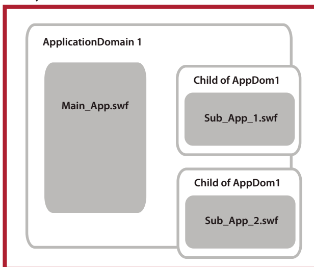
SecurityDomain 1
